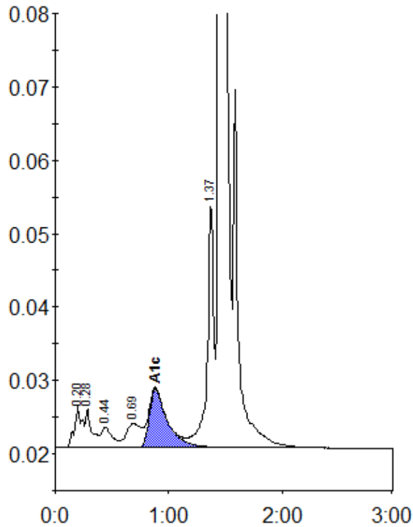
Peak table - ID: 10345261
